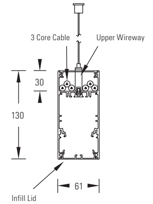
Infill/Segregated Cabling
