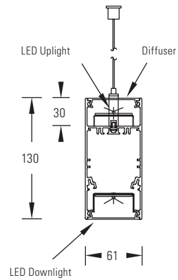
Direct/ Indirect
