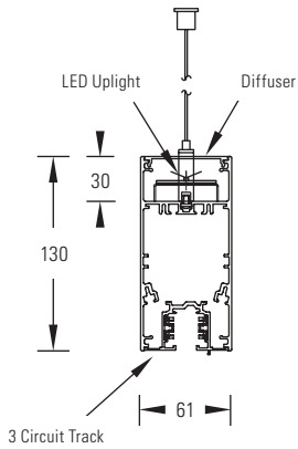
Track/ Indirect
