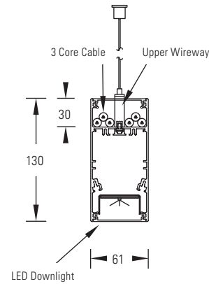
Direct/Segregated Cabling
