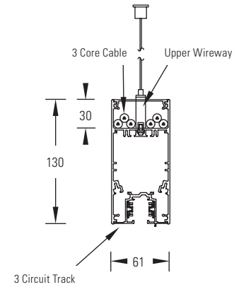
Track/Segregated Cabling
