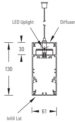
Infill/ Indirect
